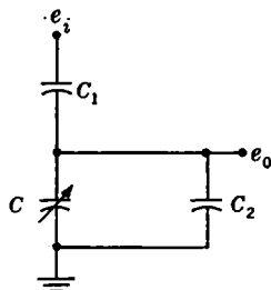
FIG. 5-35.—Condenser-divider network.
